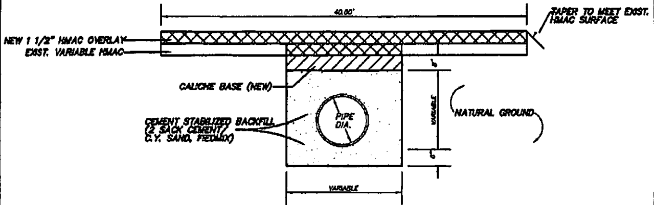
"OPEN-CUT" UTILITY ROAD CROSSING REPAIR (TYPICAL DETAIL)
